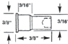
#204 RIVET FOR HARCAR VENT LOCK
