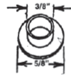
#8015 BUSHING FOR #192
