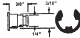
#201 1/4" RIVET & "E" RING
