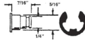
#202 1/4" RIVET & "E" RING
