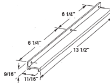
#10801 WOOD CASEMENT WINDOW REPLACEMENT TRACK
