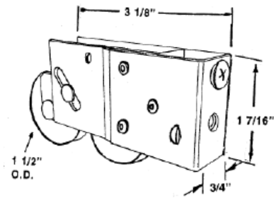
#707 TANDEM ROLLER-STEEL WHEEL #2136 STAINLESS STEEL WHEEL
