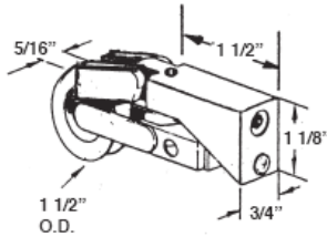
#451 KELLER PATIO ROLLER STEEL WHEEL
