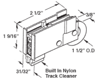
#477 ALCAN PATIO ROLLER NYLON WHEEL
