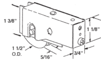
#479 LOW PROFILE PATIO ROLLER STEEL WHEEL - JONES
