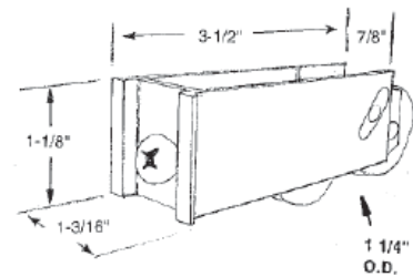
#415 R.C. ALUMINUM STAINLESS STEEL WHEEL - TANDEM
