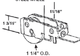
#543 AIR MASTER/LAUSELL MIRROR DOOR ROLLER STEEL WHEEL
