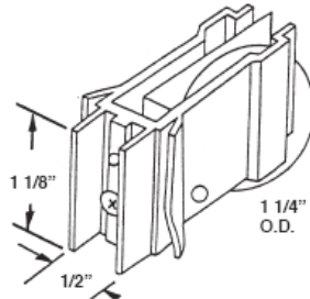
#517 THERMALUME/SUNSHINE PATIO DOOR ROLLER
