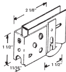
#546 PATIO DOOR ROLLER STEEL WHEEL
