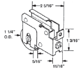
#545 LAUSELL PINO/UNIVERSAL/IMPERIAL STEEL WHEEL
