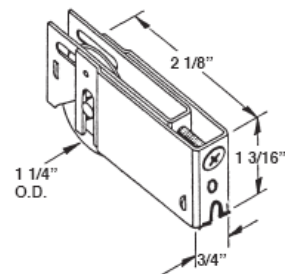
#475 NU-AIR PATIO ROLLER STEEL WHEEL
