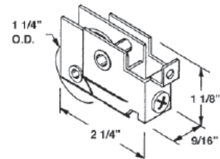
#518 DYSTON MIRROR DOOR ROLLER NYLON WHEEL
