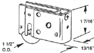
#514 BETTER-BILT PATIO ROLLER
