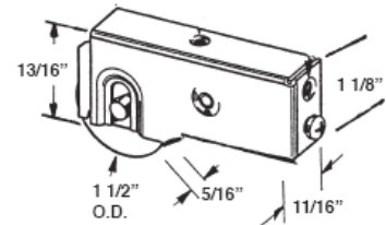
#459 PEACHTREE PATIO ROLLER
