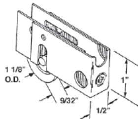
#514 BETTER-BILT PATIO ROLLER
