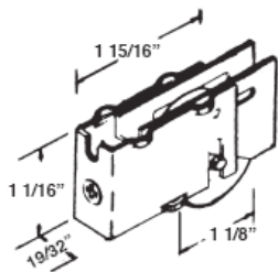
#460 CAPITAL PATIO ROLLER STEEL WHEEL
