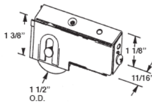
#474 LENAHAN PATIO ROLLER STEEL WHEEL #427 NYLON WHEEL
