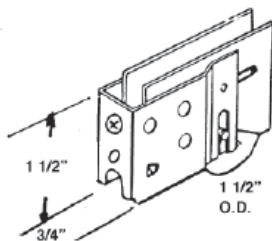
#541 AWNING WINDOW PATIO ROLLER STEEL WHEEL
