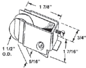
#467 LUMIDOR PATIO ROLLER NYLON WHEEL #8010 STEEL WHEEL
