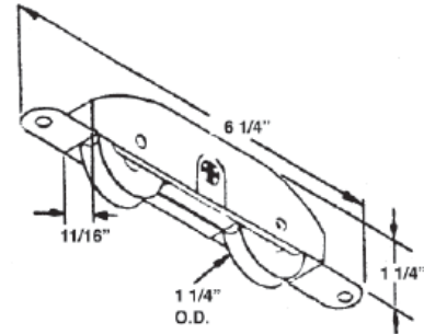
#518 DYSTON MIRROR DOOR ROLLER NYLON WHEEL
