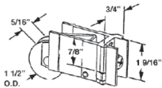
#466 LAWSON WEATHERTITE PATIO DOOR ROLLER NYLON WHEEL #466S STEEL WHEEL
