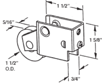
#450 AIR CONTROL PATIO ROLLER STEEL WHEEL
