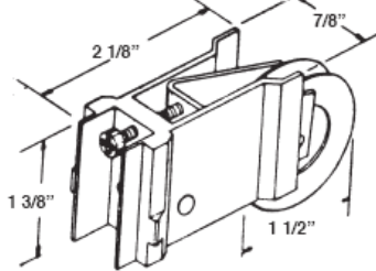
#464 PAN AM PATIO ROLLER NYLON WHEEL
