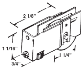
#463 DARYL-300 PATIO ROLLER STEEL WHEEL
