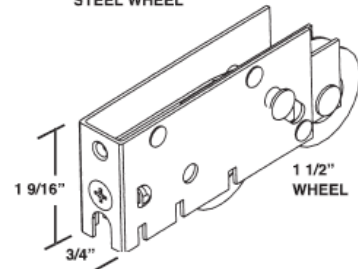
#548 HARCAR TANDEM ROLLER STEEL WHEEL
