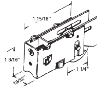
#462 ACORN PATIO ROLLER
