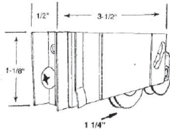
#414 THERMALUME/SUNSHINE STEEL WHEEL - TANDEM
