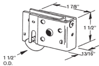
#473 PAN AM PATIO ROLLER STEEL WHEEL
