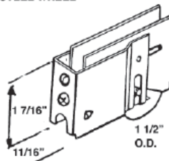
#544 TROPIC AIR PATIO ROLLER STEEL WHEEL
