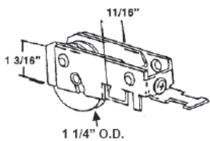
#542 AWNING WINDOW MIRROR DOOR ROLLER - STEEL WHEEL
