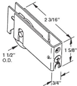
#473 PAN AM PATIO ROLLER STEEL WHEEL
