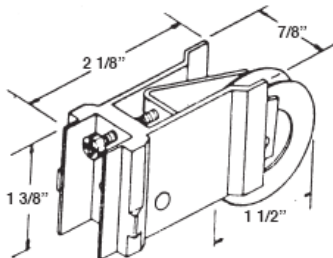
#457 PAN AM PATIO ROLLER STEEL WHEEL
