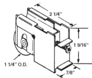
#462 ACORN PATIO ROLLER
