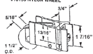
#10083 WALLACE PATIO ROLLER STEEL WHEEL #10133 NYLON WHEEL
