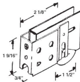
#461 CROWN/LAWSON PATIO ROLLER
