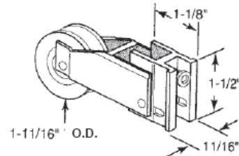
#456 PLAZA DOOR/DARYL PM NYLON WHEEL
