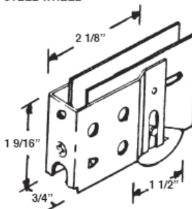
#458 HARCAR/PGT PATIO ROLLER STEEL WHEEL
