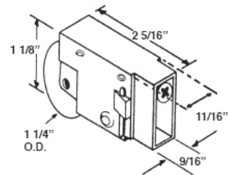
#476 CROSSLY PATIO ROLLER STEEL WHEEL
