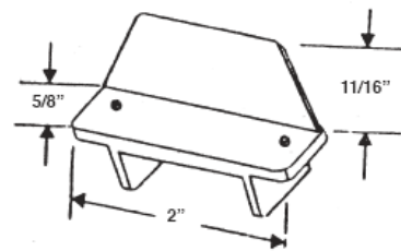
#422 DRAWER BRACKET & WHEEL GUIDE
