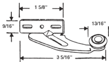
#421 DRAWER BRACKET & WHEEL
