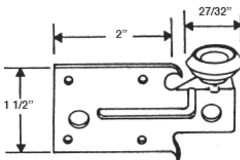
#411 DRAWER BRACKET & WHEEL
