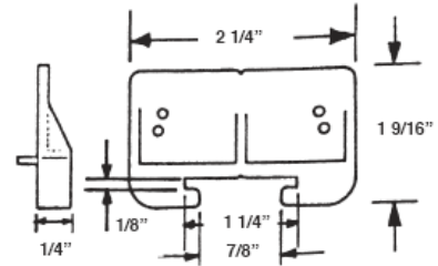
#425 NYLON DRAWER SLIDE
