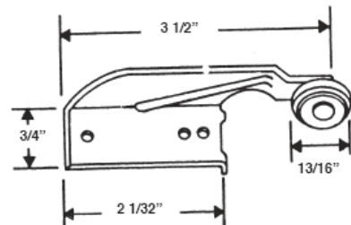
#422 DRAWER BRACKET & WHEEL GUIDE
