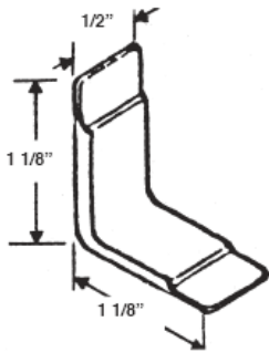
#417 TRACK REAR BRACKET
