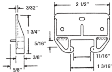
#420 DRAWER TRACK SLIDE GUIDE
