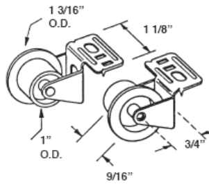
#420 DRAWER TRACK SLIDE GUIDE
