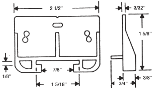
#407 DRAWER NYLON SLIDE
