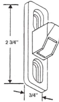
#488 STANDARD KEEPER
