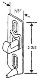
#490 CROSSLY KEEPER
