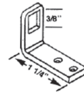
#485 DARYL KEEPER
