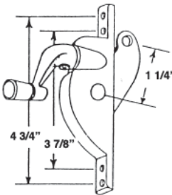
#787 LUDMAN OPERATOR L.H.
