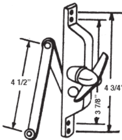
#257 SUPERIOR JALOUSIE OPERATOR
