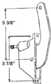
#787 LUDMAN OPERATOR L.H.
