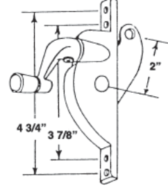
#791 D-8 L.H. JTW OPERATOR
