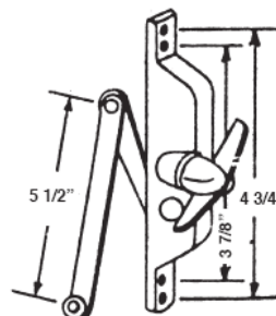
#260 5 1/2" JALOUSIE OPERATOR
