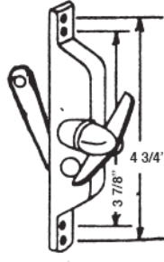
#261 UNIVERSAL JALOUSIE OPERATOR
