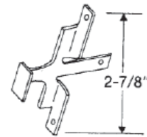
#10407 AIRPLANE LATCH
