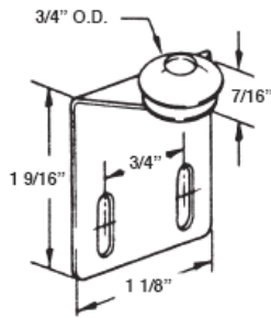
#630 SCREEN DOOR ROLLER ASSY STEEL WHEEL
