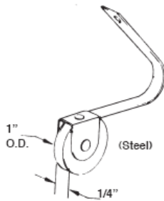
#562 SLIDING SCREEN DOOR ROLLER ASSY
