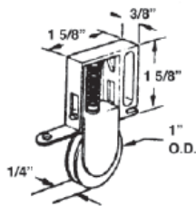
#665 SCREEN DOOR ROLLER ASSY NYLON WHEEL
