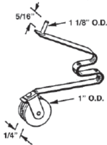
#628 "W" ROLLER WITH PIN NYLON WHEEL
