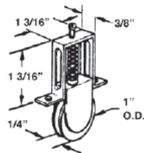
#666 SCREEN DOOR ROLLER ASSY NYLON WHEEL
