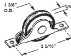
#1000 GARAGE DOOR SCREEN ROLLER
