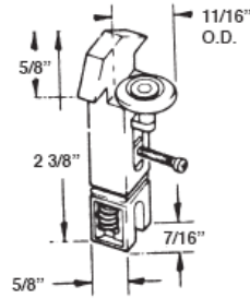
#573 SLIDING SCREEN DOOR ROLLER ASSY
