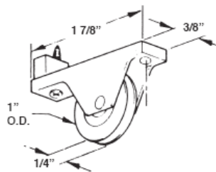
#569 SLIDING SCREEN DOOR ROLLER ASSY
