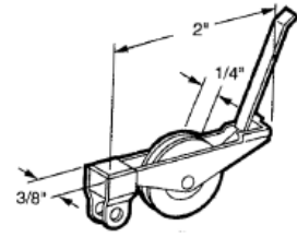
#76 MSC SCREEN DOOR WHEEL ASSY
