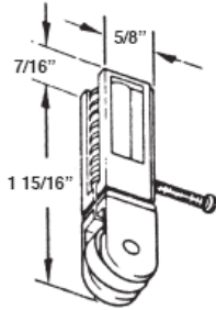
#572 SLIDING SCREEN DOOR ROLLER ASSY
