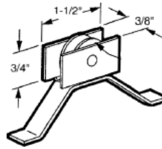
#75 KELLER SCREEN DOOR WHEEL ASSY
