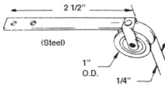
#630 SCREEN DOOR ROLLER ASSY STEEL WHEEL
