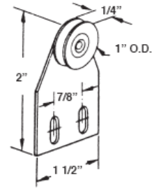
#576 SLIDING SCREEN DOOR ROLLER ASSY
