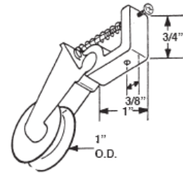
#561 SLIDING SCREEN DOOR ROLLER ASSY - NYLON WHEEL
