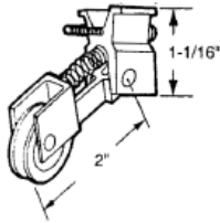
#81 JONES SCREEN DOOR WHEEL ASSY
