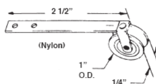
#631 SCREEN DOOR ROLLER ASSY NYLON WHEEL
