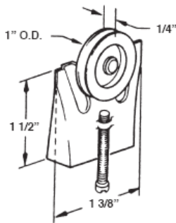
#631 SCREEN DOOR ROLLER ASSY NYLON WHEEL
