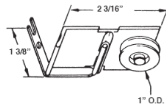
#635 SCREEN DOOR ROLLER ASSY
