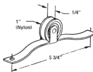
#569 SLIDING SCREEN DOOR ROLLER ASSY
