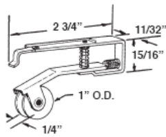
#81 JONES SCREEN DOOR WHEEL ASSY
