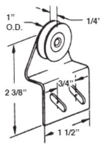
#574 SLIDING SCREEN DOOR ROLLER ASSY
