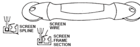
#652 DOUBLE WHEEL TOOL METAL HANDLE
