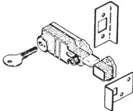
#174 SINGLE HUNG WINDOW LOCK
