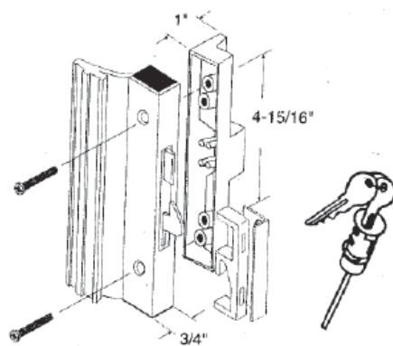
#446 UNIVERSAL SURFACE MOUNT LOCK SET WITH KEY
