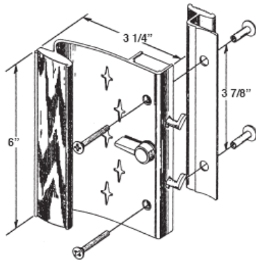
#447 UNIVERSAL SURFACE MOUNT LOCK SET
