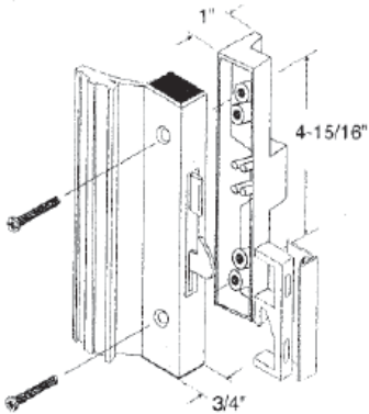
#447 UNIVERSAL SURFACE MOUNT LOCK SET
