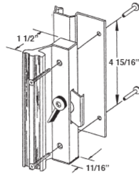
#446 UNIVERSAL SURFACE MOUNT LOCK SET WITH KEY
