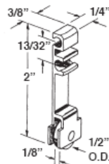
#10619 HORIZONTAL WINDOW LATCH
