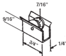
#399 HORIZONTAL WINDOW ROLLER ASSY
