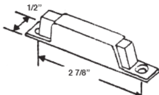
#10229 AIR CONTROL HORIZONTAL LATCH
