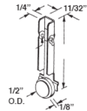
#9205 STAMPED METAL WITH NYLON WHEEL
