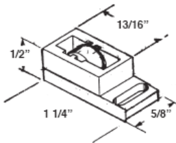
#10229 AIR CONTROL HORIZONTAL LATCH
