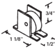
#393 HORIZONTAL WINDOW ROLLER ASSY
