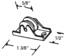
#390 HORIZONTAL WINDOW ROLLER ASSY
