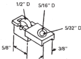
#9203 WITH BRASS WHEEL
